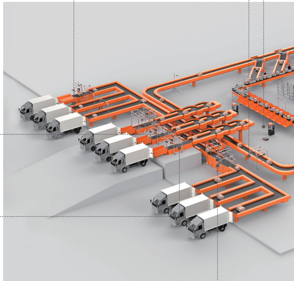
Dynamic Scanning & Positioning System
