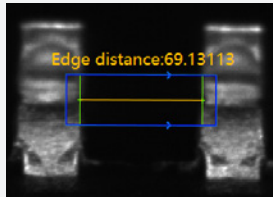
Edge distance measurement
