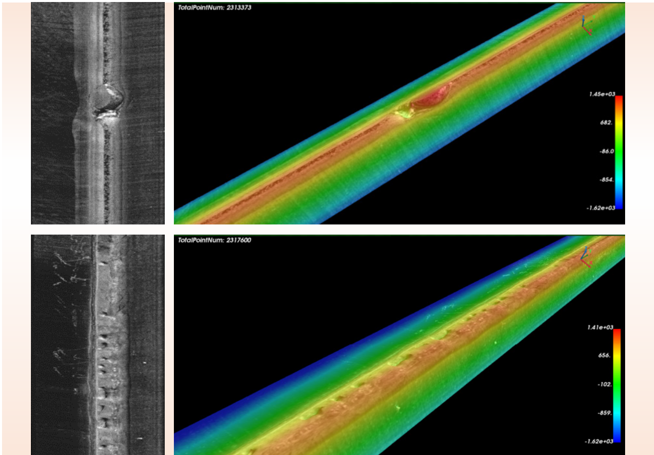
Defect detection of the welding treatment of the top cover perimeter
