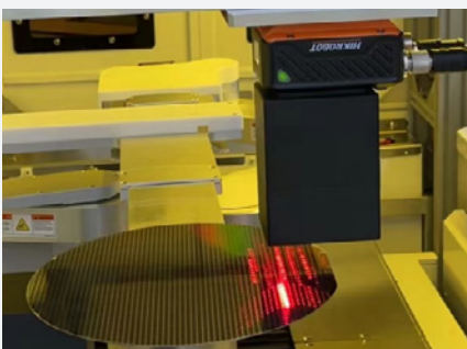
Silicon wafer SEMI font recognition
