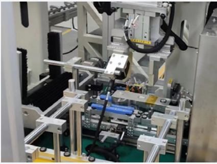
Battery top cover laser-engraved code reading
