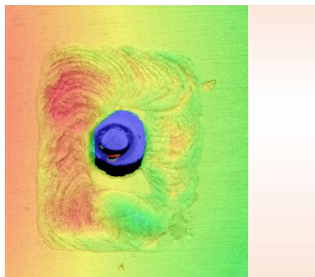
Defect detection of the busbar welding
