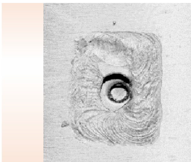
Defect detection of the busbar welding
