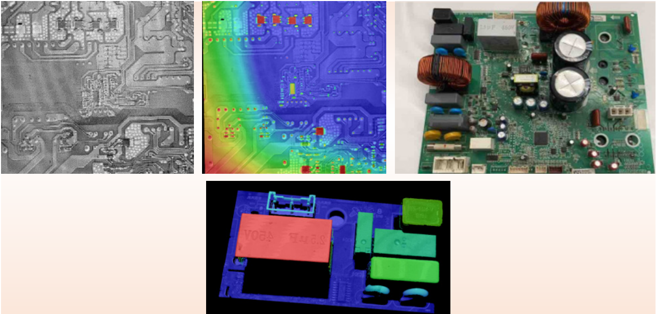
Height detection of the PCB parts
