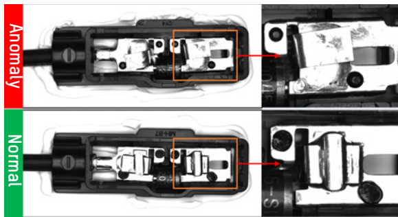
PV module junction box welding scar detection: using deep learning with traditional detection algorithms to detect PV module junction box welding scars.
