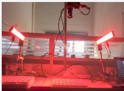
Consumer electronic parts batch code reading
