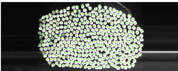
Rebar counting: Use deep learning algorithm to implement counting function when rebar is bundled.
