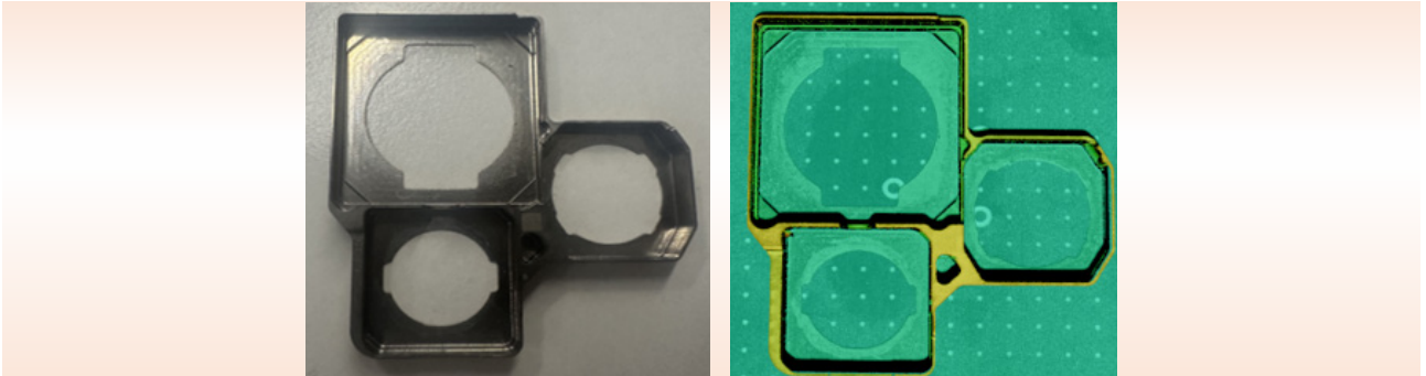
Measurement of step and coplanarity of folds in mobile phone camera modules
