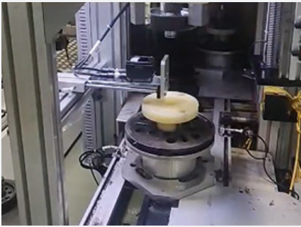
Gear DPM code reading
