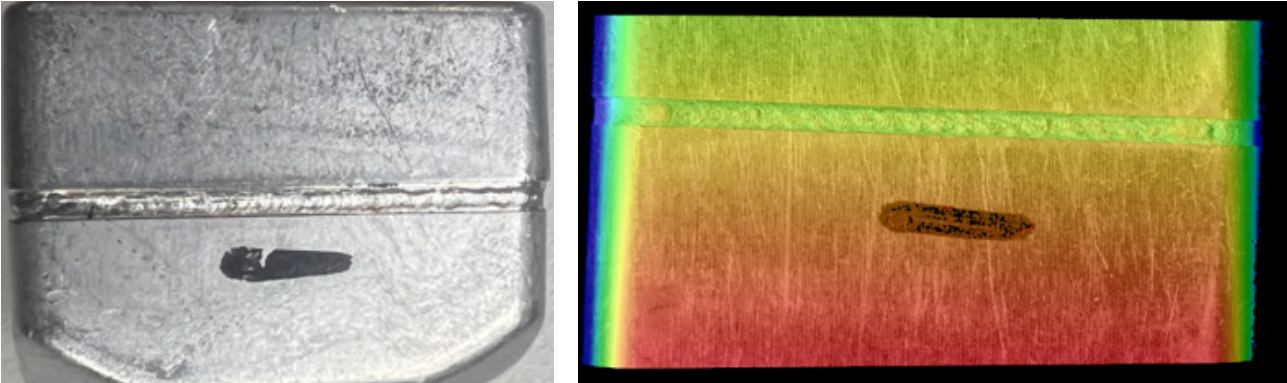
Defect detection of structural part welding seam
