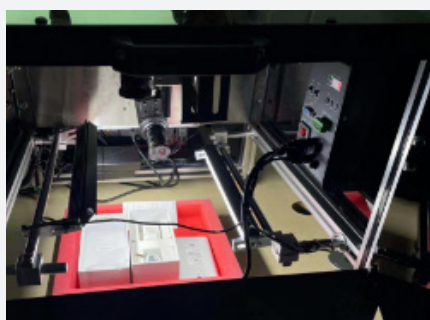
Phone package code reading
