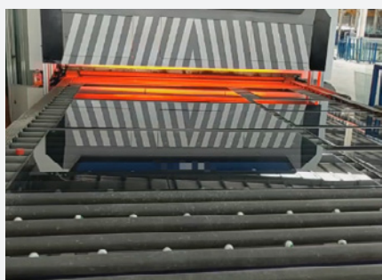
Large-field of view code reading in glass industry
